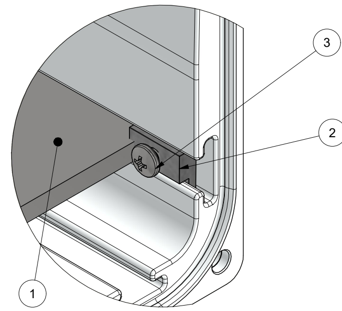
DETAIL A
